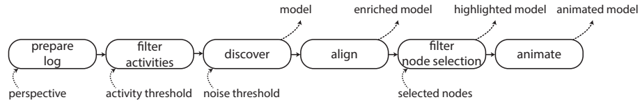
Figure 2: Chain of tasks, their parameters (bottom) and their visual results (top). If a user changes a parameter, the necessary tasks restart immediately.
